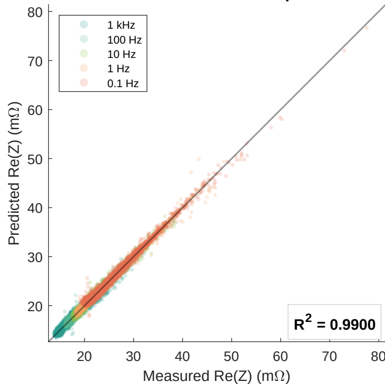
Predicted vs measured impedance
